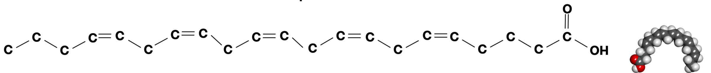
Eicosapentaenoic acid
