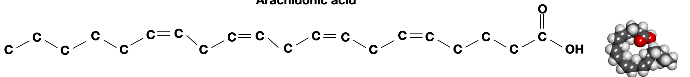
Arachidonic acid
