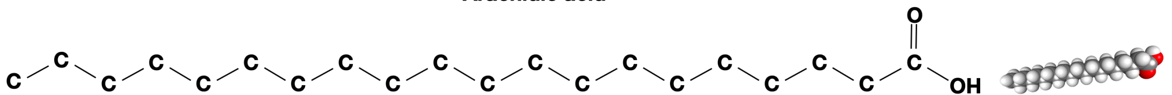
Arachidic acid
