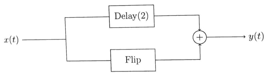
Figure 2: System for Problem 2(3).
